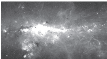
The Peony nebula star was found in the crowded, dusty center of our Milky Way galaxy, seen here in a false-color infrared view from NASA's Spitzer Space Telescope.
